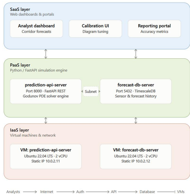
Figure 1: End-to-End Cloud System Architecture and Service Model Mapping (IaaS / PaaS / SaaS)
